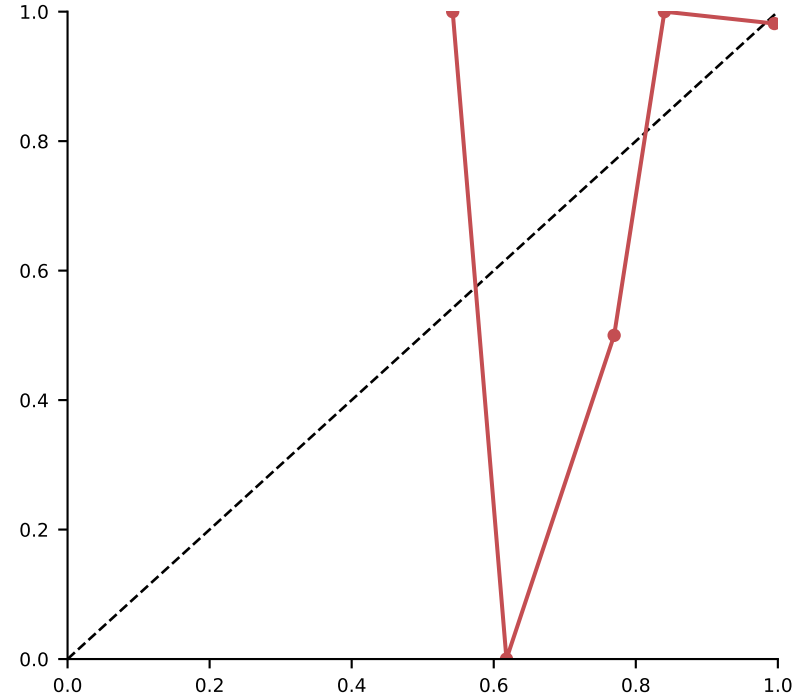
Has_RBC ECE=0.031, n=230
